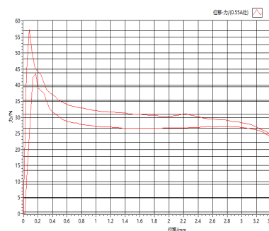
F-S characteristic curve
